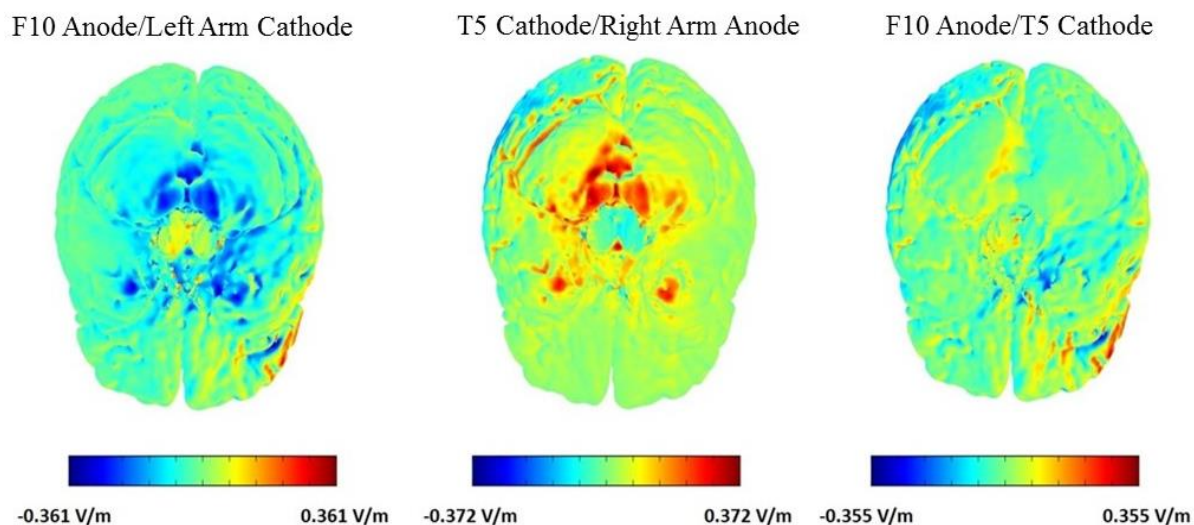
Figure 2: Current modeling. Finite element models show F10 (left) or T5 (middle) vs. shoulder placements produce large effects in the cerebellum with opposite polarities, whereas a bicephalic F10 anode vs. T5 cathode (right) does not.
