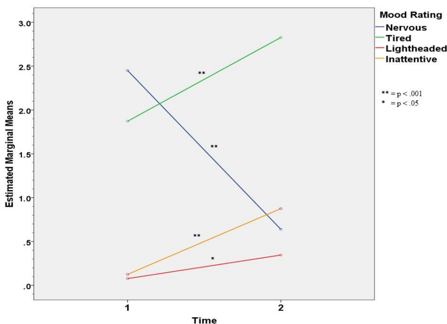
Figure 15. Changes in self-reported mood ratings. Feelings of nervousness were significantly higher before training and stimulation than after, collapsed across groups, while feelings of tiredness, lightheadedness and inattentiveness were significantly increased after training and stimulation compared to baseline.
